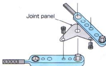
Joint panels (optional attachments)
